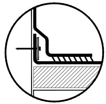
SECUREMENT FASTENED AT BASE OF WALL OR CURB ALTERNATE BASE FASTENING
